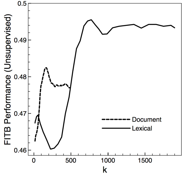
Figure 1: FITB Performance on different LoAs as a function of the latent space dimensionality.
