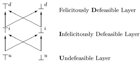
Figure 1: The lattice that underlies stratified logic
