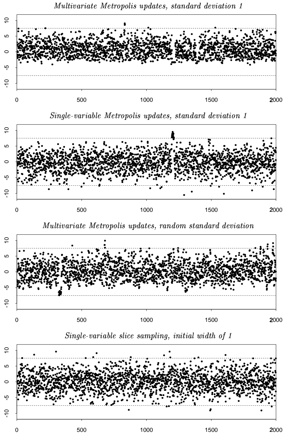
FIG. 14. Sampling from the funnel distribution using Metropolis and slice-sampling methods.
