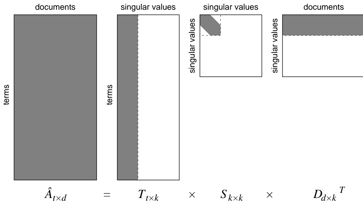
Figure 1.2: Approximate recomposition of a matrix
