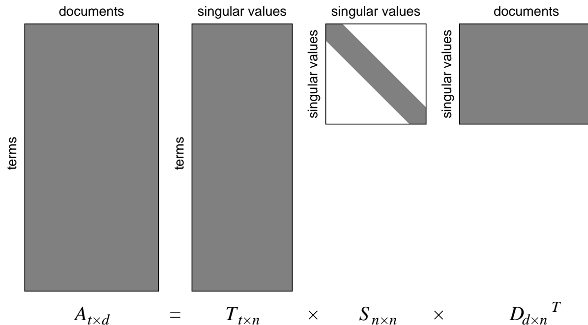
Figure 1.1: Singular value decomposition of a matrix
