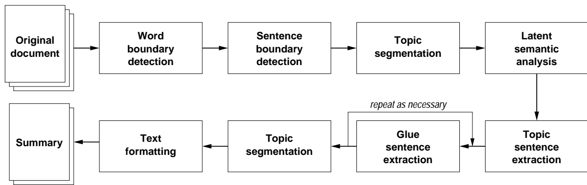
Figure 2.1: Summarizer architecture
